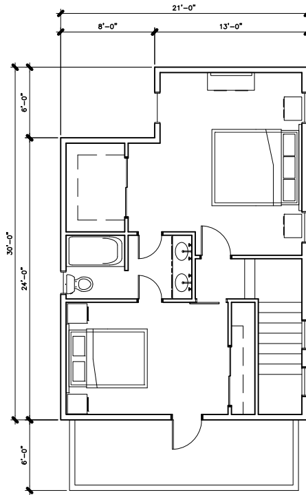
02 SECOND FLOOR PLAN 1/8"=1'-0" 582 SQ FT
