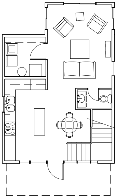
01 FIRST FLOOR PLAN 1/8"=1'-0" 582 SQ FT
